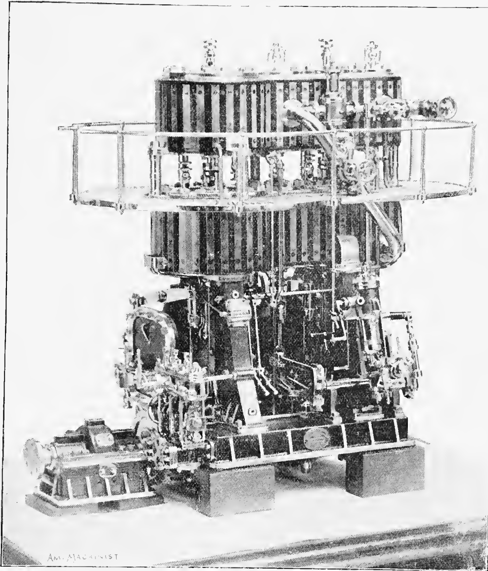
CHASE'S QUADRUPLE-EXPANSION MARINE ENGINE.
